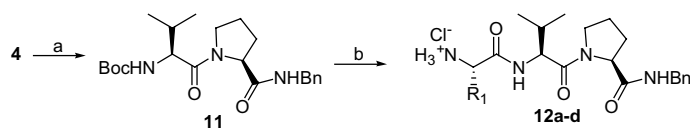
Scheme 2. Synthesis of peptido-mimetics with modifications at Ala residue. Reagents and conditions: (a) i. 2N LiOH, 1,4-dioxane, then 1N HCl, ii. benzylamine, EDC, HOBt, N,N -diisopropylethylamine, \text{CH}_2\text{Cl}_2 , 88% over two steps; (b) i. 4N HCl in 1,4-dioxane, MeOH, ii. L - N -Boc-amino acid, EDC, HOBt, N,N -diisopropylethylamine, \text{CH}_2\text{Cl}_2 , iii. 4N HCl in 1,4-dioxane, MeOH, structures are shown in Table 1, the yield over three steps is 68–74%.
