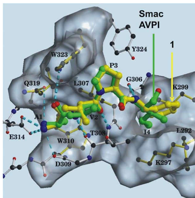
Figure 1. Superposition of modeled structure of compound 1 (yellow) complexed with XIAP BIR3 and the X-ray structure of Smac protein (green) complexed with XIAP BIR3. Compound 1 in complex with XIAP BIR3 was modeled based upon the X-ray structure of XIAP BIR3 in complex with Smac and minimized using the Sybyl program. 23 For clarity, only the AVPI residues of Smac are shown. Carbon atoms are colored in yellow, green and black in compound 1, Smac AVPI peptide, and in the protein, respectively. Nitrogen and oxygen atoms in these molecules are colored in blue and red, respectively. Hydrogen bonds are depicted in blue dashed lines.
