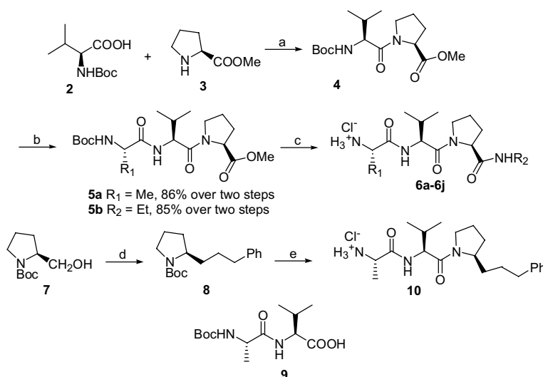
Scheme 1. Synthesis of peptido-mimetics with modifications at Ile residue. Reagents and conditions: (a) EDC, HOBT, N,N -diisopropylethylamine, \text{CH}_2\text{Cl}_2 , 92%; (b) i. 4N HCl in 1,4-dioxane, MeOH, ii. L-N-Boc-alanine or L-N-Boc-aminobutyric acid, EDC, HOBT, N,N -diisopropylethylamine, \text{CH}_2\text{Cl}_2 ; (c) i. 2N LiOH, 1,4-dioxane, then 1N HCl, ii. amine, EDC, HOBT, N,N -diisopropylethylamine, \text{CH}_2\text{Cl}_2 , iii. 4N HCl in 1,4-dioxane, MeOH, structures were shown in Table 1, the yield over three steps is 48–72%; (d) i. Dess–Martin periodinane, \text{CH}_2\text{Cl}_2 , ii. phenylethyltriphenylphosphonium bromide, n -BuLi, -78^\circ\text{C} , THF, iii. 10% Pd–C, \text{H}_2 , 51% over three steps; (e) i. 4N HCl in 1,4-dioxane, MeOH, ii. 9 , EDC, HOBT, N,N -diisopropylethylamine, \text{CH}_2\text{Cl}_2 , 4N HCl in 1,4-dioxane, MeOH, 72% over three steps.
