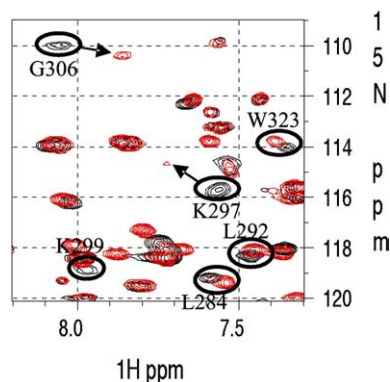
Figure 2. Overlaid ^{15}\text{N} heteronuclear single quantum coherence spectroscopy (HSQC) NMR spectra of XIAP BIR3 with (red) or without (black) compound 6j .
